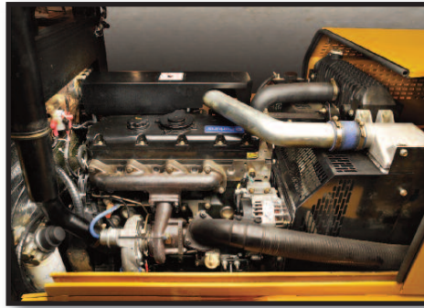
ENGINE: The unique sliding hood provides unobstructed engine access for quick maintenance checks. A Perkins Tier 3 Turbo Diesel is standard.
