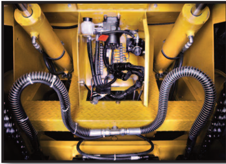
MAINTENANCE PANEL: Electrical, steering, and brake maintenance is facilitated through a hinged compartment located at the front of the unit.
